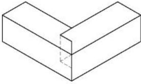
13-1. 반연귀맞춤
