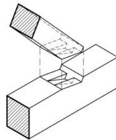
12. 흘림장부안장맞춤
