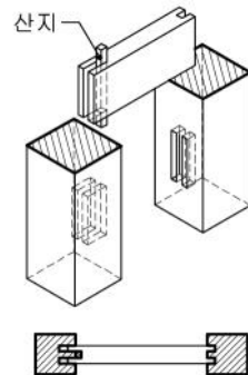
3. 뒤맞춤
